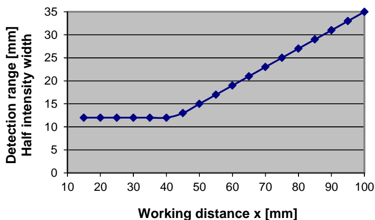
SPECTRO-3-30-FCL Detection range [mm]
