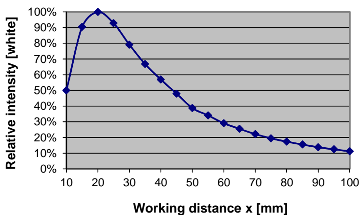
SPECTRO-3-50-POL INT [relative]
