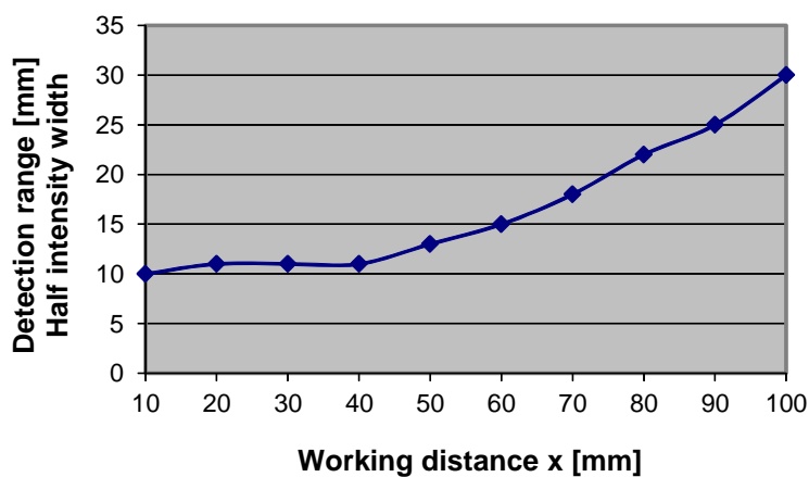
SPECTRO-3-50-POL Detection range [mm]
